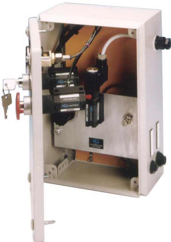
Cabinet for filling machine
