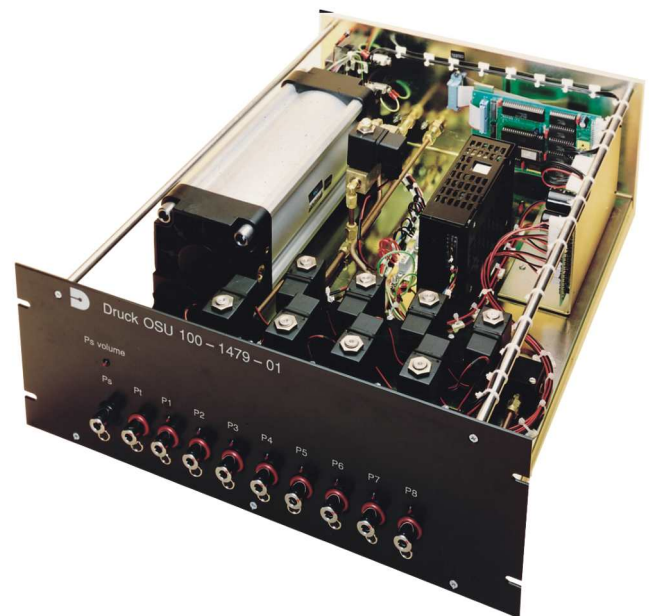
Customised cabinet 'rack' system for aerospace industry
