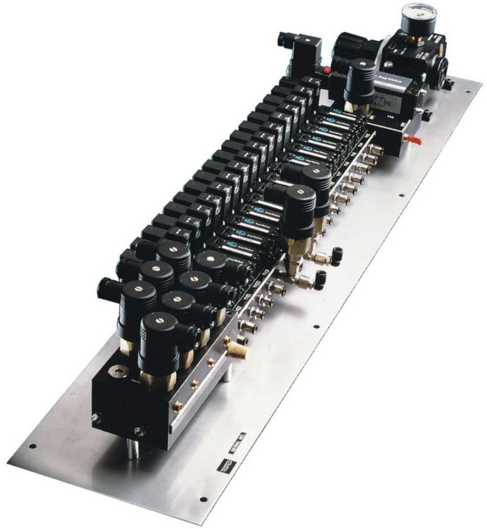
Sub-plate system for pharmaceutical machine
